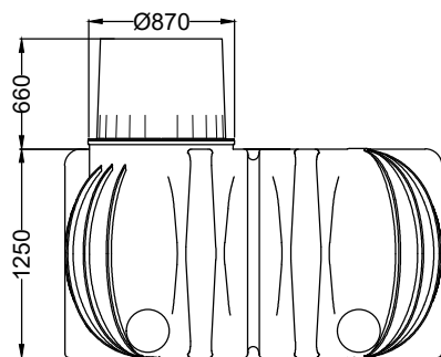
View A
