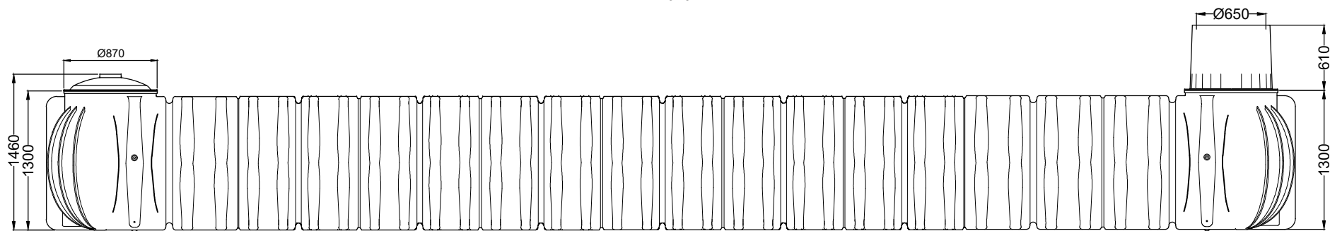
View A
