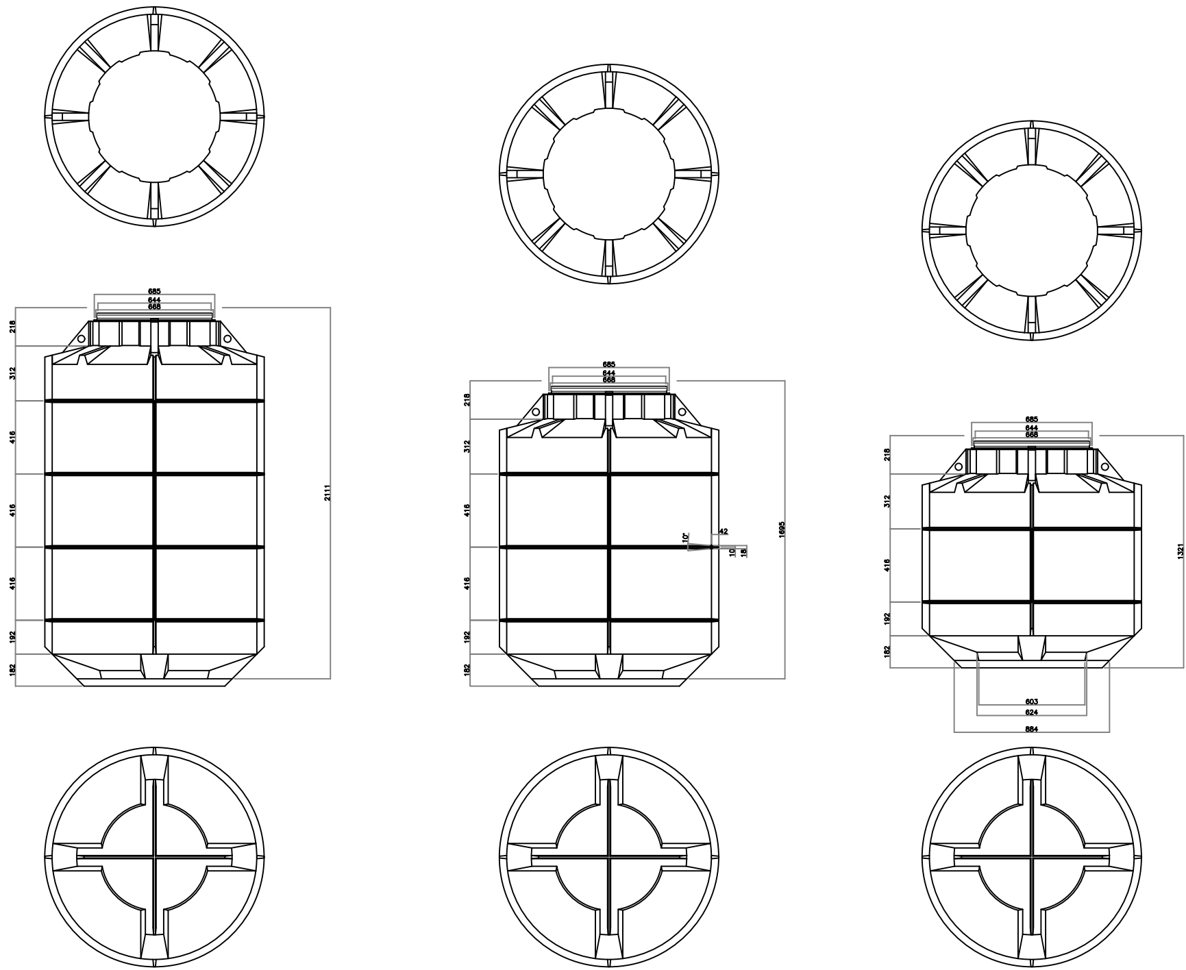
MOULDS — NO FLANGES SHOWN FOR CLARITY
