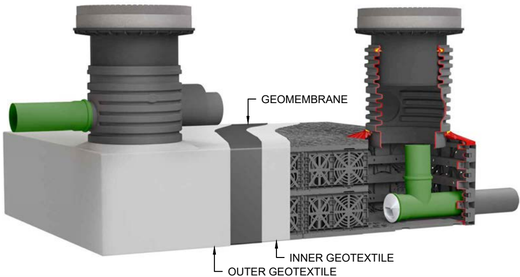
Connector clips are Red for illustration purposes only and are Grey in colour
