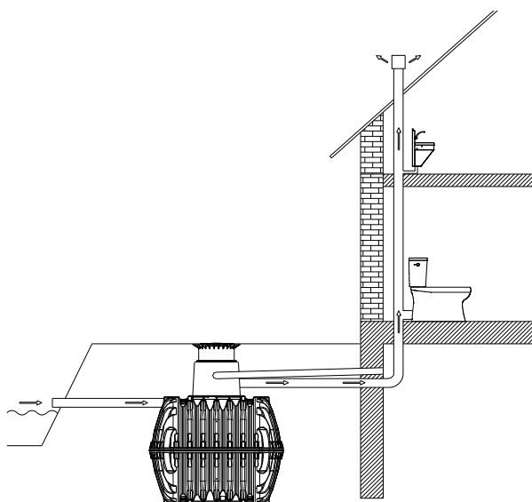
Ventilation with free discharge
