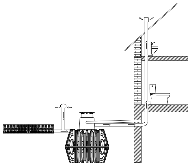
Ventilation with seepage or discharge not free
